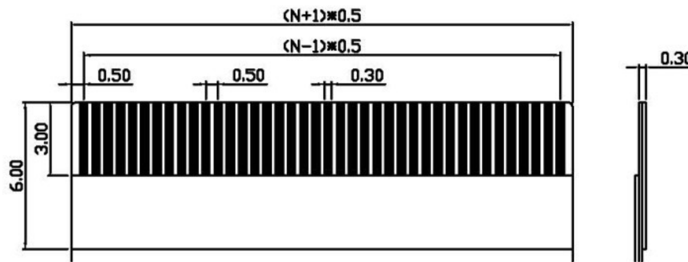
RECOMMENDED FFC/FPC DIM.
