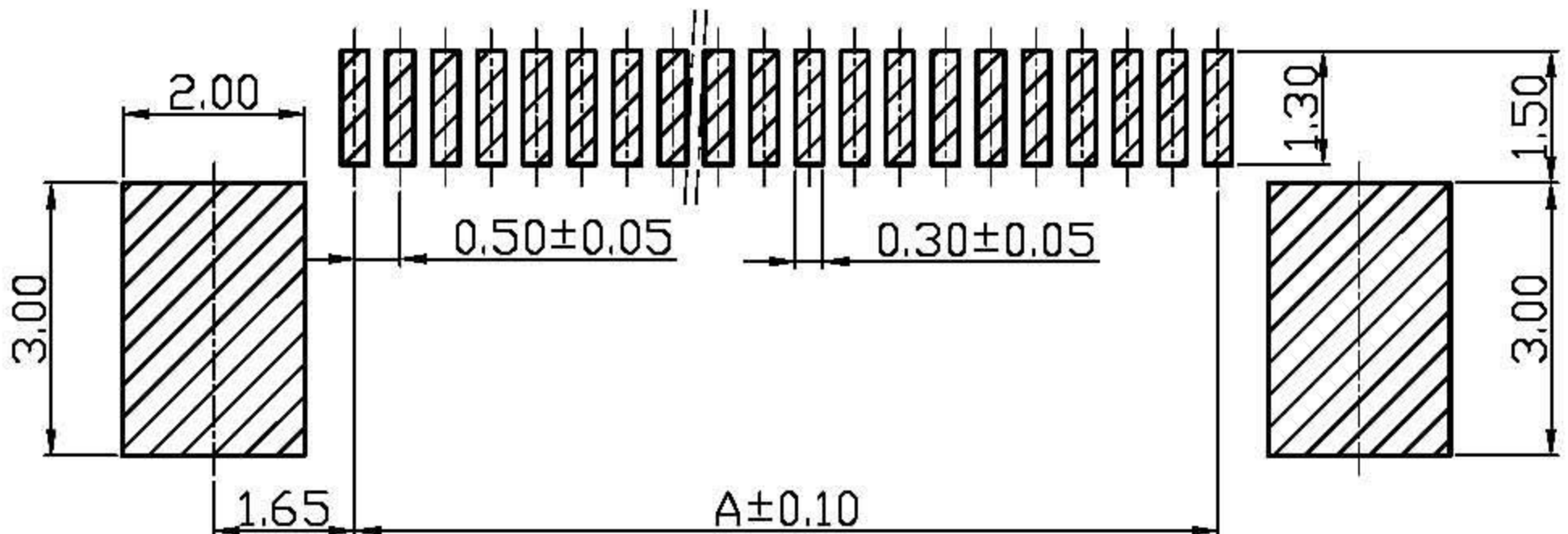
PCB Layout
