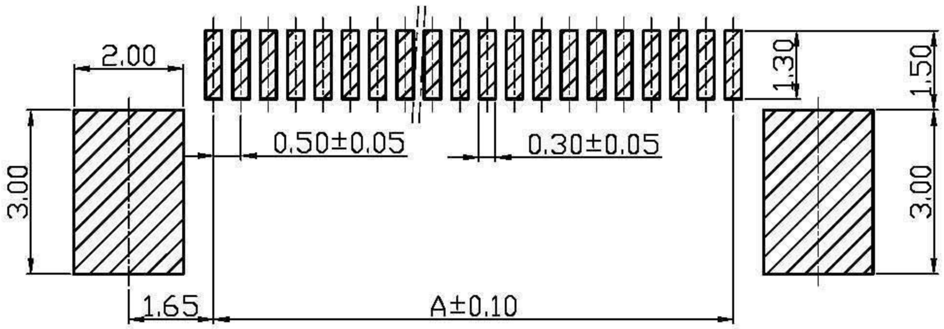
PCB Layout
