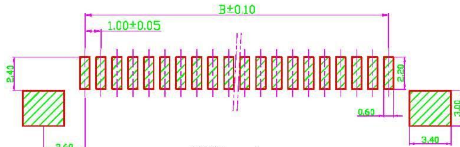
PCB Layout
