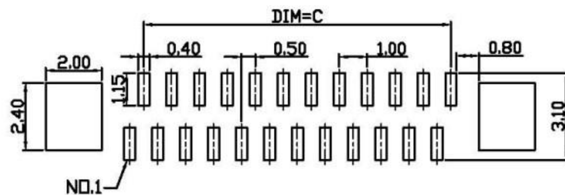
RECOMMENDED P.C.B LAYOUT NEGATIVE-NEEDLE CIRCUIT BOARD
