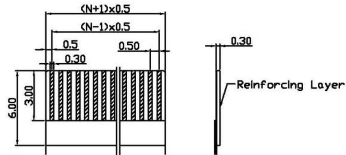
RECOMMENDED FFC/FPC DIM
