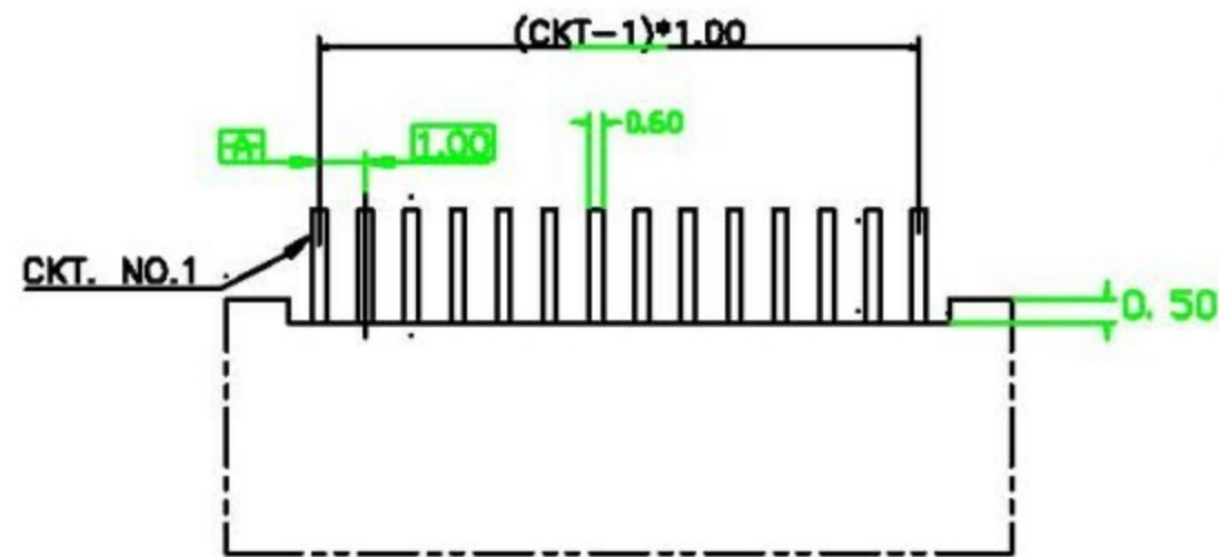
PC BOARD LAYOUT TOP VIEW
