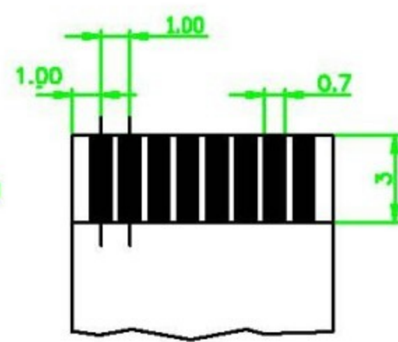
FFC/FPC DIMENSION THICKNESS 0.26~0.32mm TOLERANCE: 0.05mm
