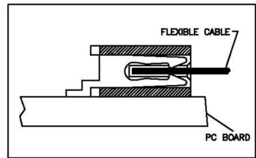
Q-Q SECTION
