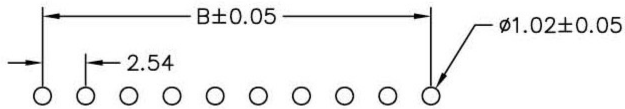
Recommended P.C.B Layout
